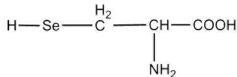
Selenocystein
