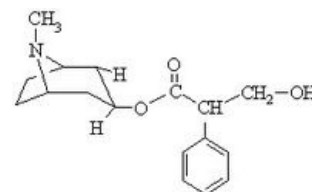
Atropin
