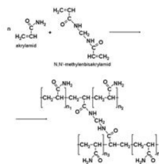
Polyakrylamid
