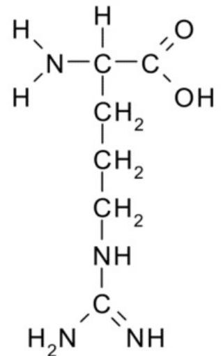
Arginin
