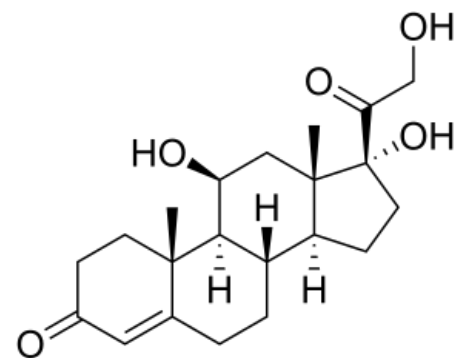
Chemical formula of cortisol
