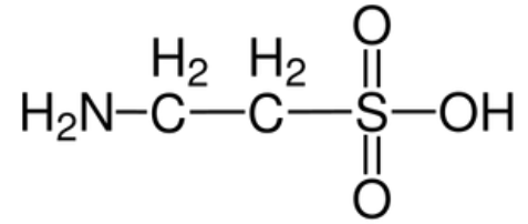
The structural formula of taurine
